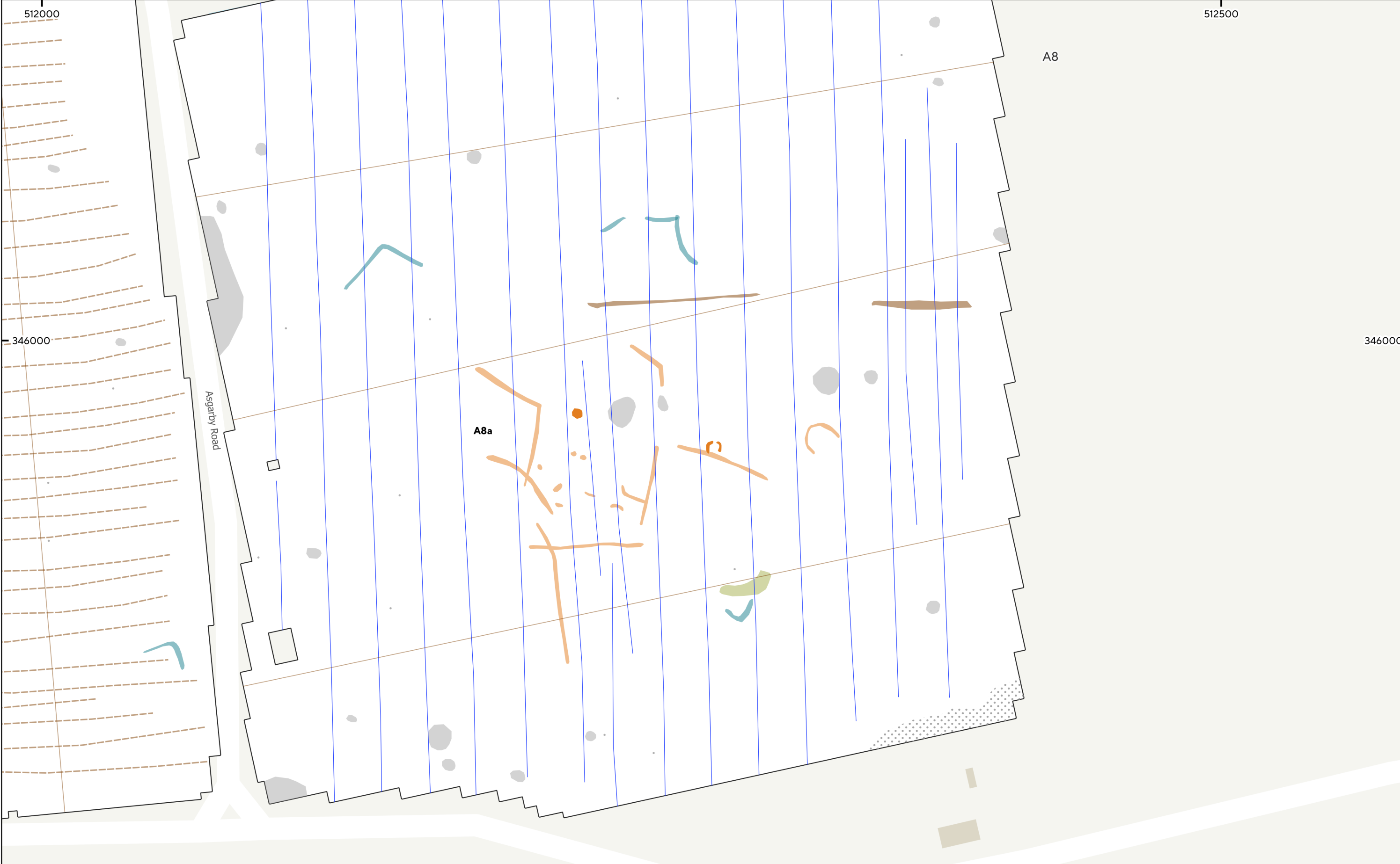
MSTF1735 - Beacon Fen Cable Route, Lincolnshire Figure 119 - Magnetic Interpretation (Area of Archaeological Activity 9 - Areas A7-A8) 1:1,500 @ A3 © Magnitude Surveys 2024 Contains Ordnance Survey data © Crown Copyright and database right 2024
