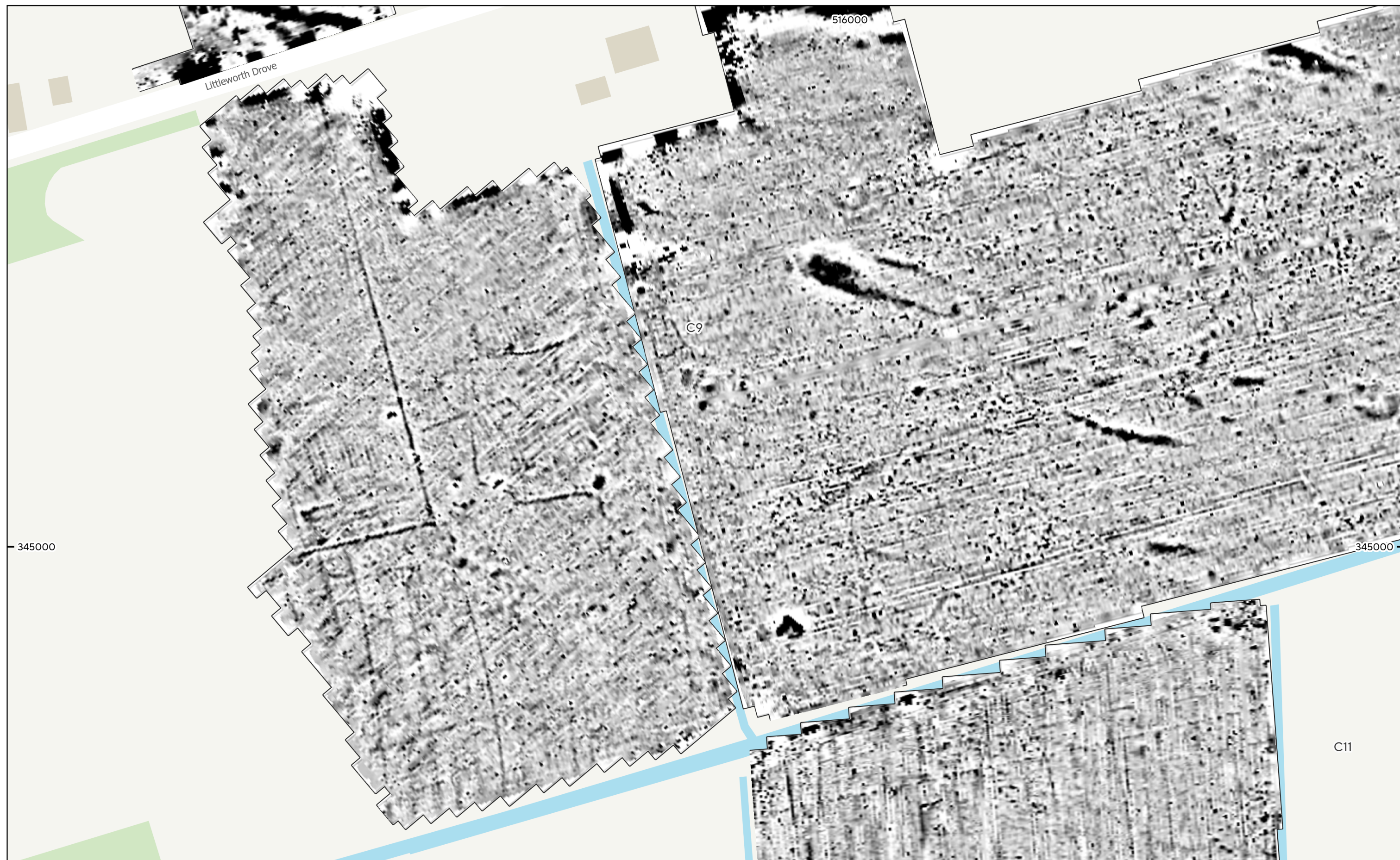
MSTF1735 - Beacon Fen Cable Route, Lincolnshire Figure 121 - Magnetic Gradient (Area of Archaeological Activity 10 - Area C9) 1:1,500 @ A3 © Magnitude Surveys 2024 Contains Ordnance Survey data © Crown Copyright and database right 2024
