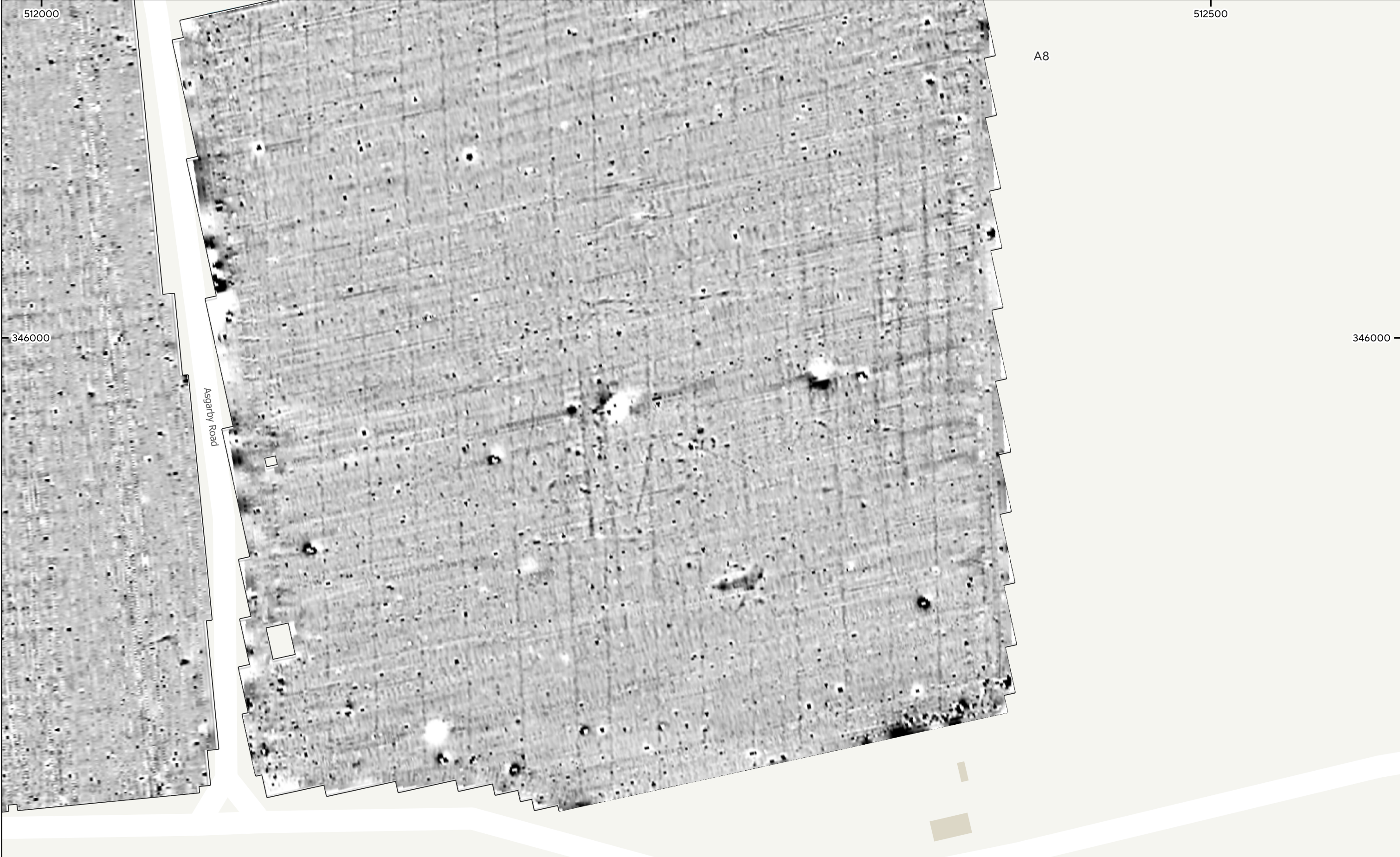
MSTF1735 - Beacon Fen Cable Route, Lincolnshire Figure 118 - Magnetic Gradient (Area of Archaeological Activity 9 - Areas A7-A8) 1:1,500 @ A3 © Magnitude Surveys 2024 Contains Ordnance Survey data © Crown Copyright and database right 2024
